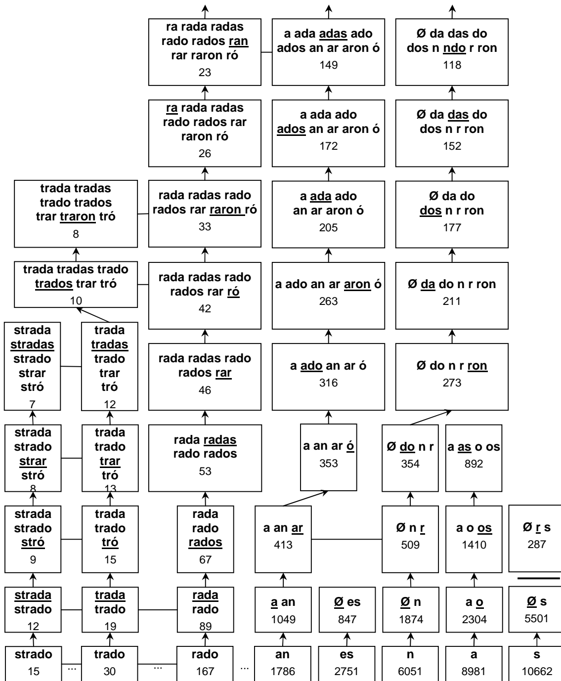
Figure 2: Eight search paths that ParaMor follows in search of likely partial paradigms. Search paths begin at the bottom of the figure and move upward. Candidate suffixes appear in bold . The underlined candidate suffix in each partial paradigm is the suffix added by the most recent search step. Each partial paradigm gives the number of candidate stems which attach to all candidate suffixes in that partial paradigm. Horizontal links between partial paradigms connect sets of suffixes that differ only in their initial character.
